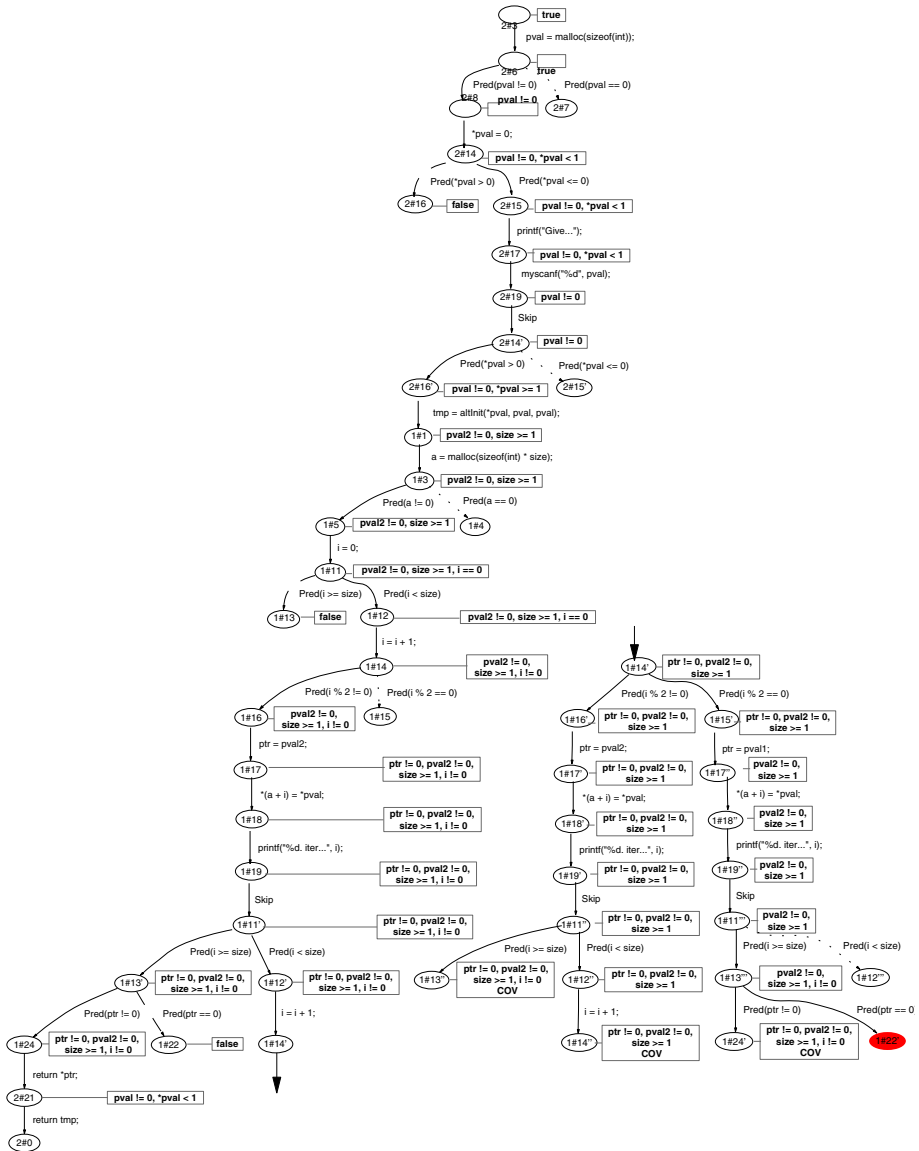
Fig. 8. Abstract reachability tree when the third spurious error path is found
