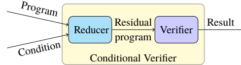
Fig. 1: Reducer-based conditional verifier template
